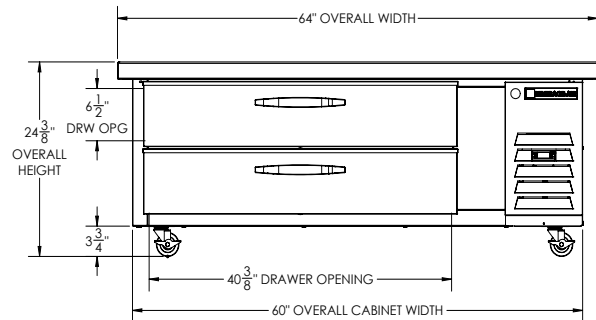
ELEVATION VIEW
