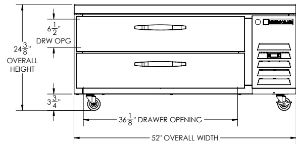
ELEVATION VIEW
