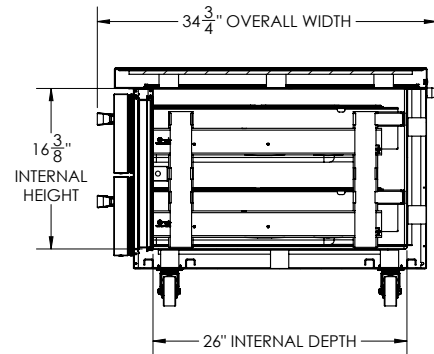
ELEVATION VIEW
