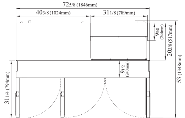
TST-72SD-08S-N-CL-LW TOP VIEW
