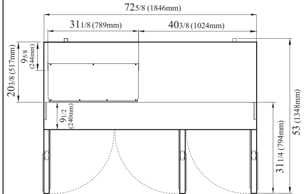
TST-72SD-08S-N-CL TOP VIEW
