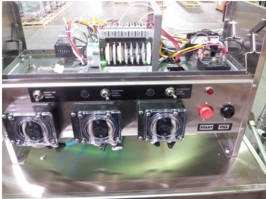
Showing control box, chemical pumps, prime switches
