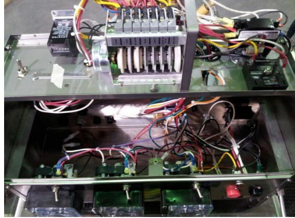
Showing AWS control tray lifted to service pumps
