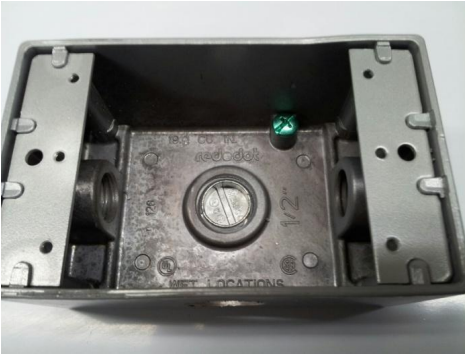
Ground screw in junction box
