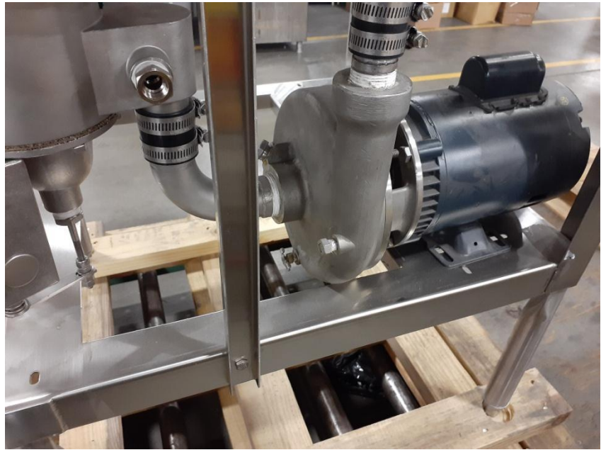
Wash Pump and Motor
