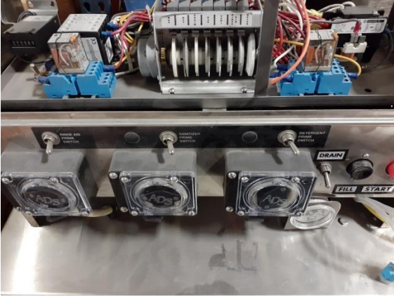
Showing AWS-H control tray in normal position
